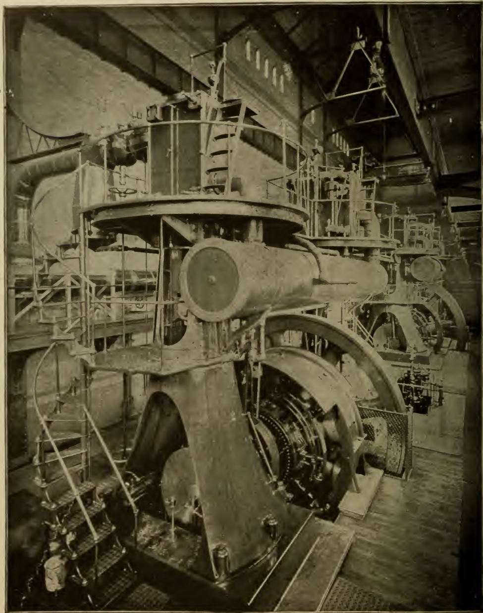
Fig. 18. SCENE IN THE METROPOLITAN ELEVATED POWER HOUSE, CHICAGO, ILL. 800 and 1500 Kilowatt Direct-Driven Railway Generators.
